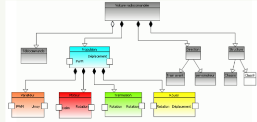
Block definition
