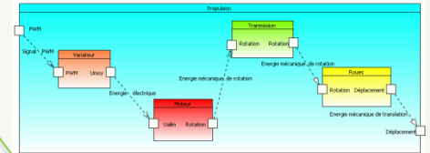
Internal Block
